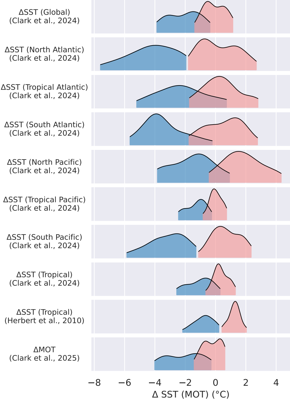
(b) SST + MOT records
