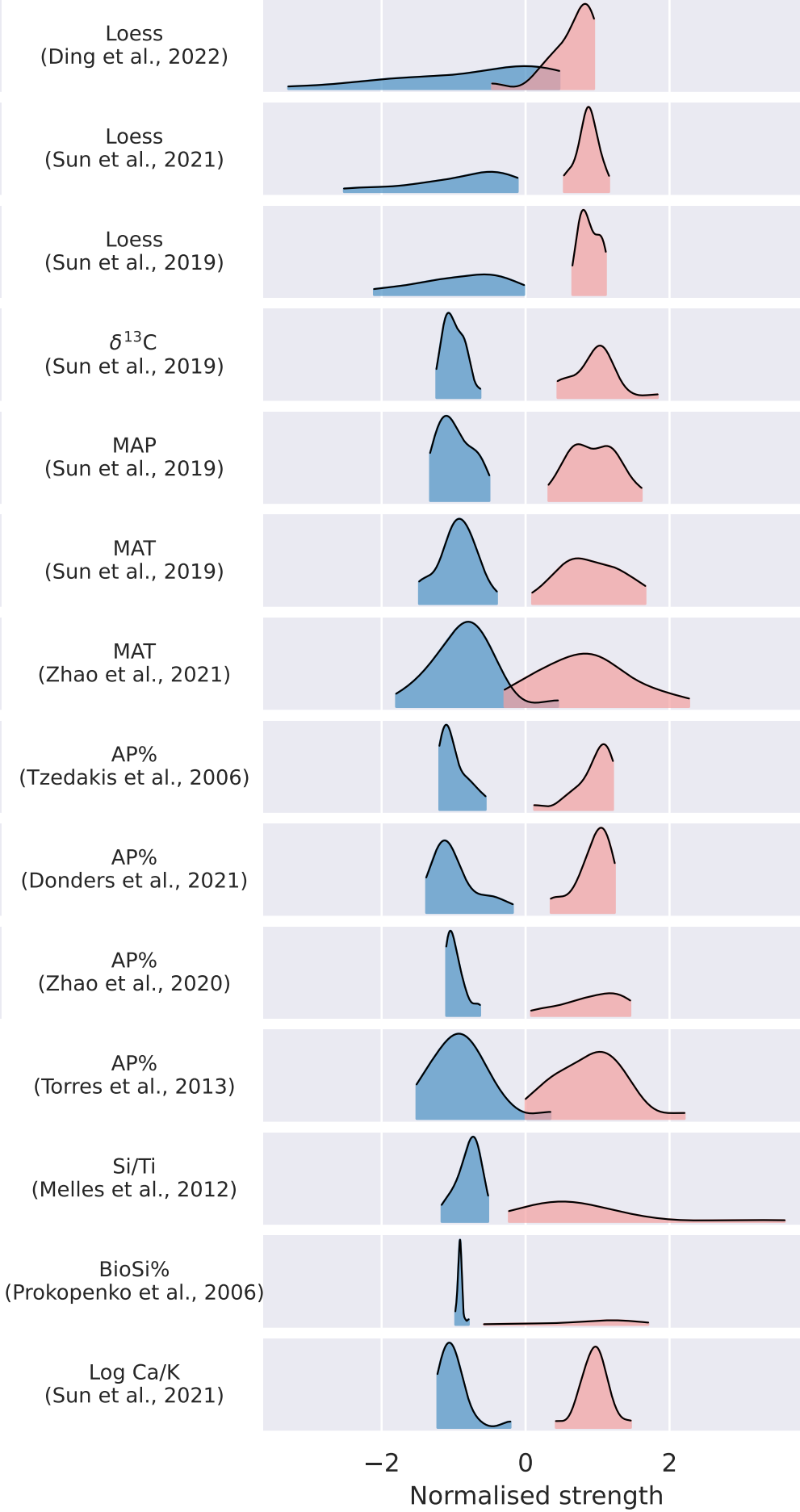
(c) Terrestrial records
