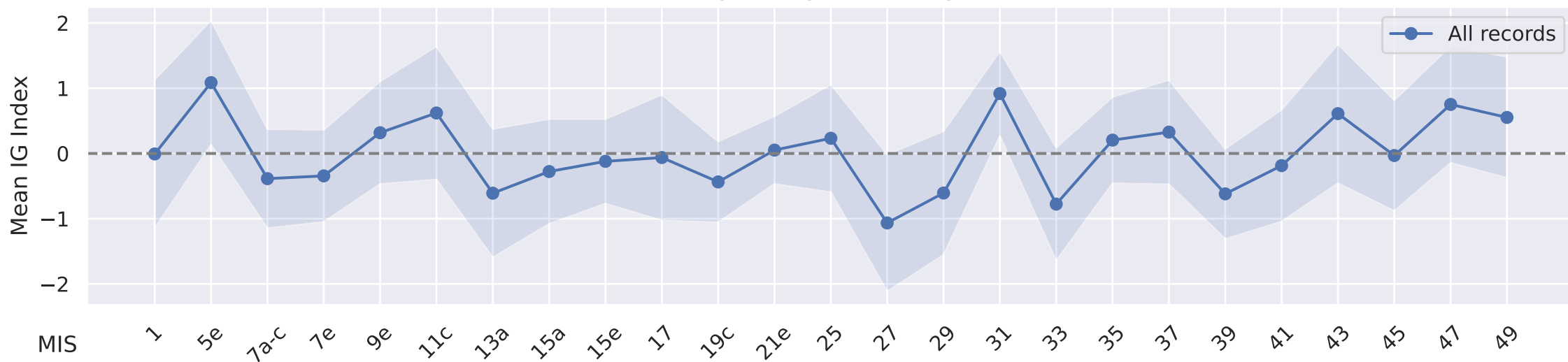
(a) Average Interglacial Strength Index
