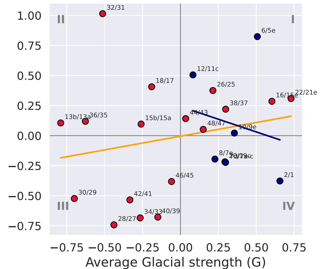
(c) Terrestrial Records
