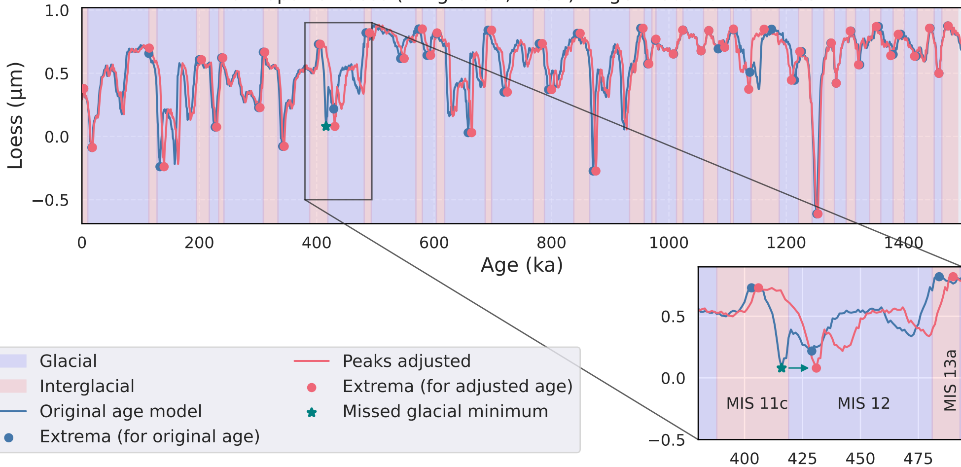
Chiloparts Loess (Ding et al., 2002) - Age model differences
