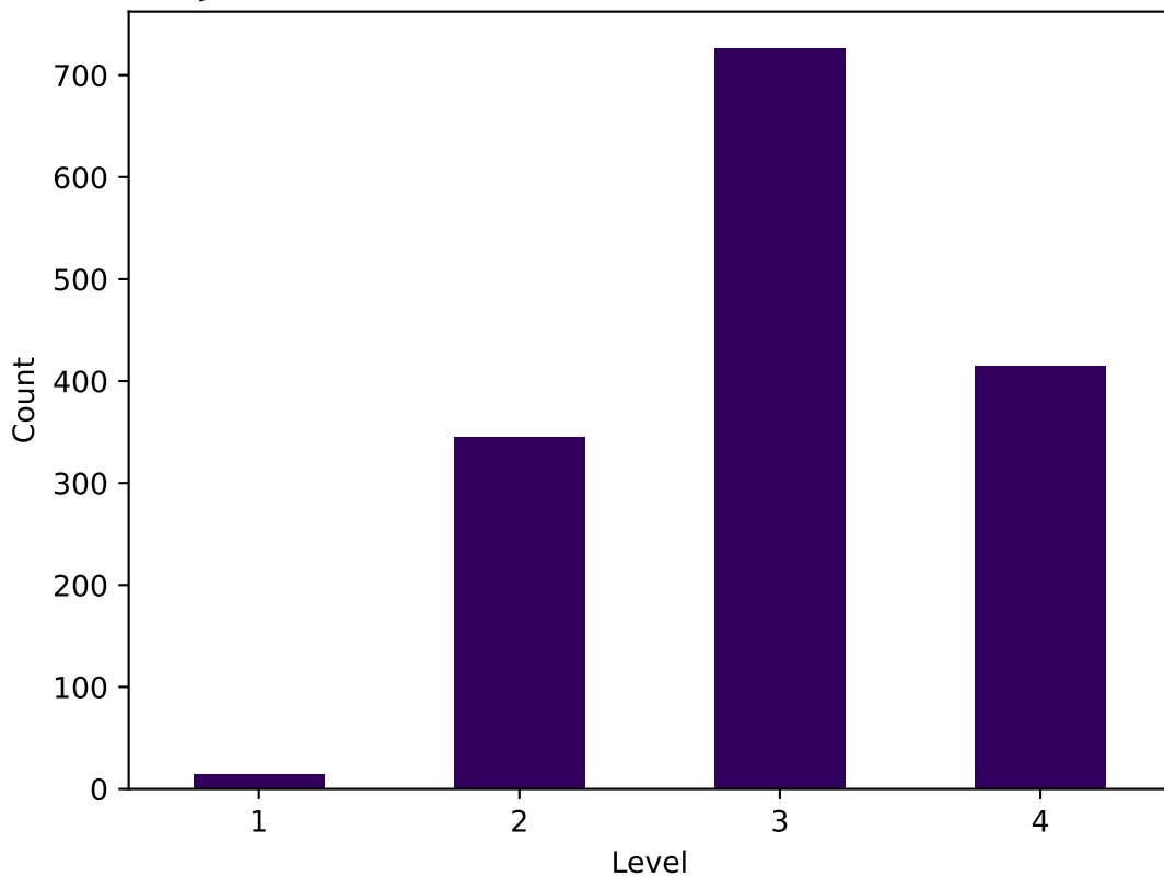
Object Detection Demand-Level Distribution (calibration)
