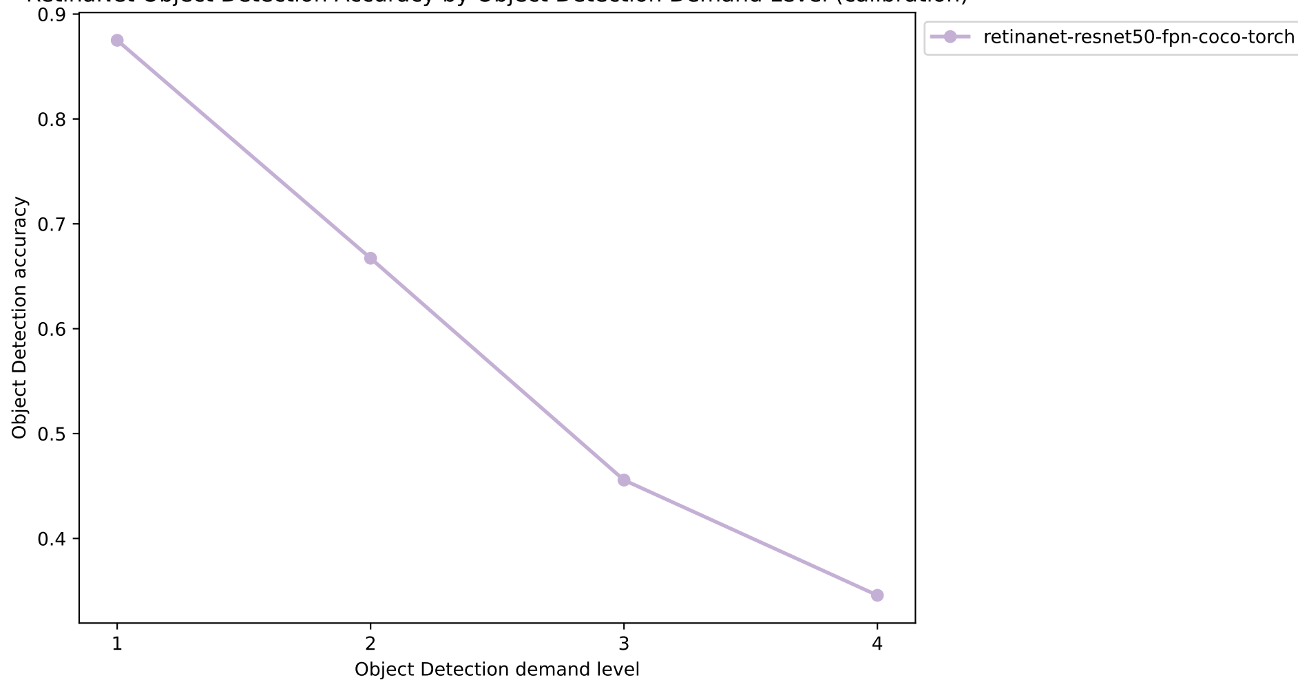
RetinaNet Object Detection Accuracy by Object Detection Demand Level (calibration)
