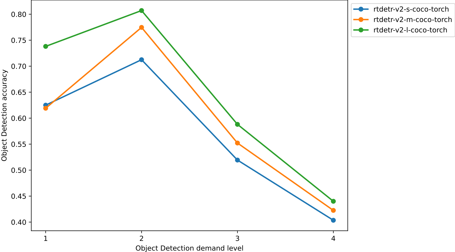
RT-DETRv2 Object Detection Accuracy by Object Detection Demand Level (calibration)
