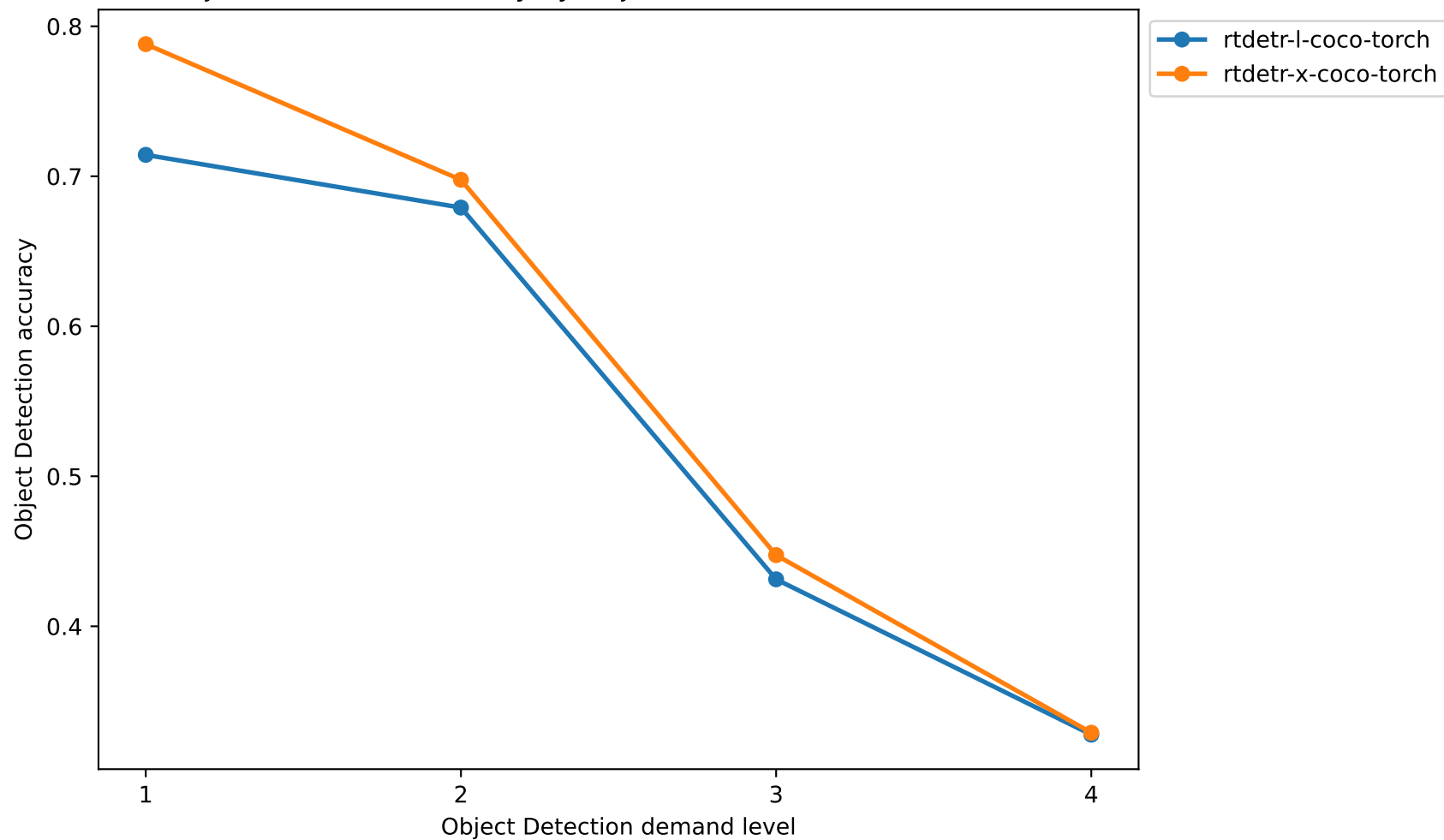
RT-DETR Object Detection Accuracy by Object Detection Demand Level (calibration)
