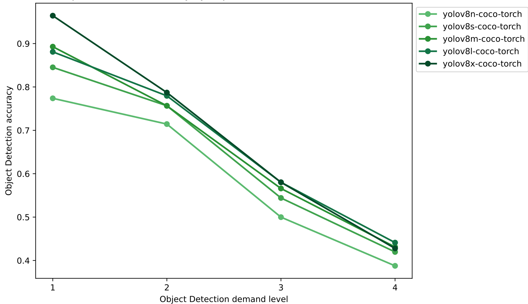
YOLOv8 Object Detection Accuracy by Object Detection Demand Level (calibration)
