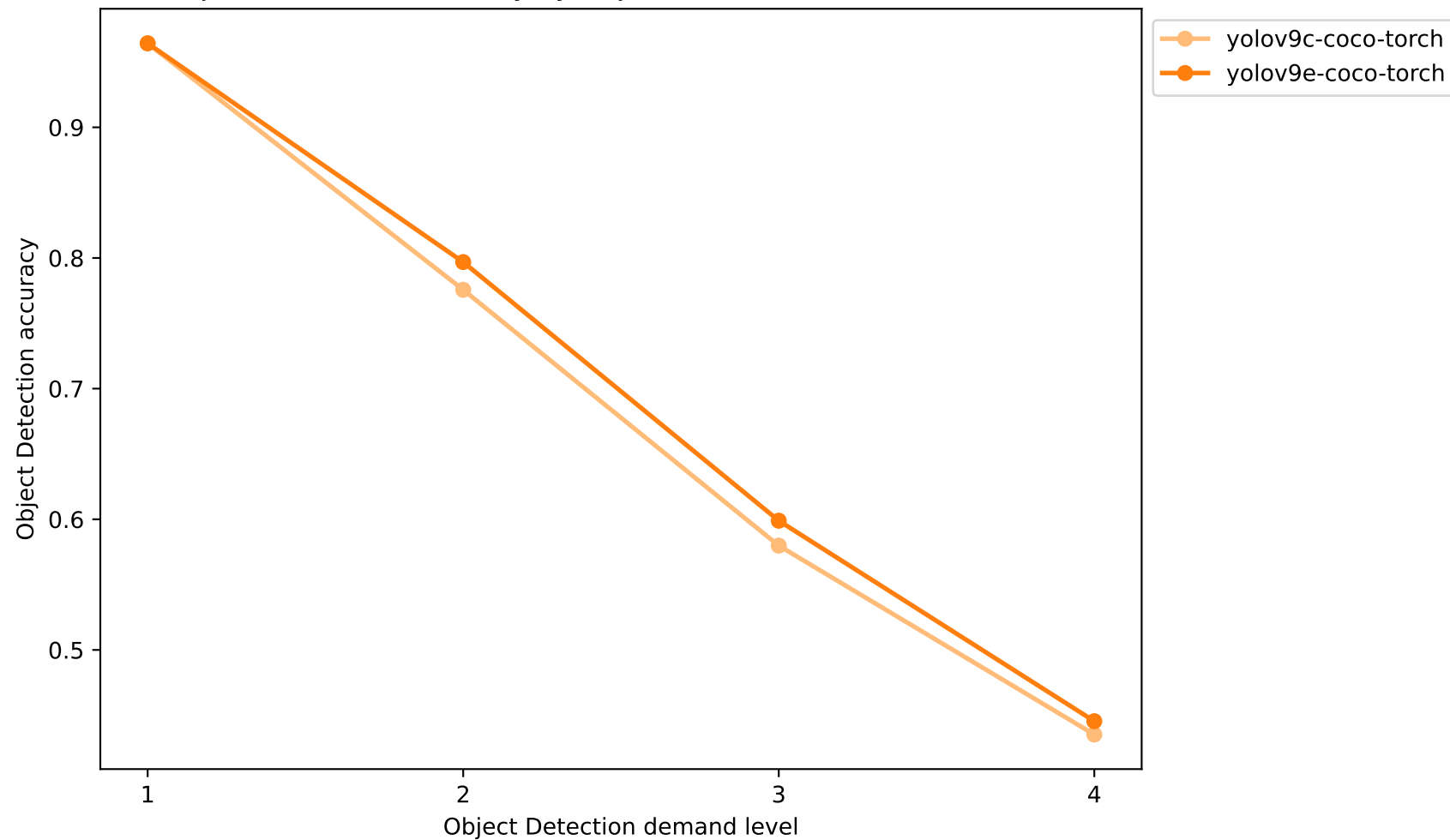
YOLOv9 Object Detection Accuracy by Object Detection Demand Level (calibration)
