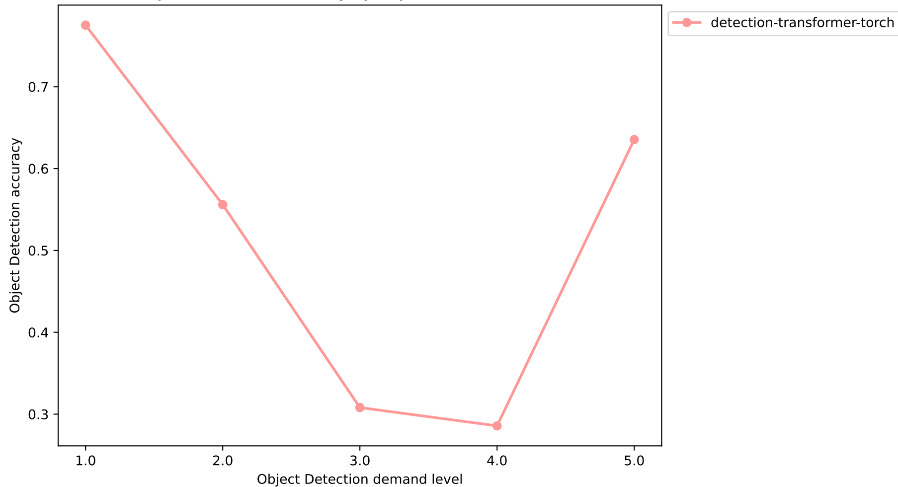
DETR Object Detection Accuracy by Object Detection Demand Level
