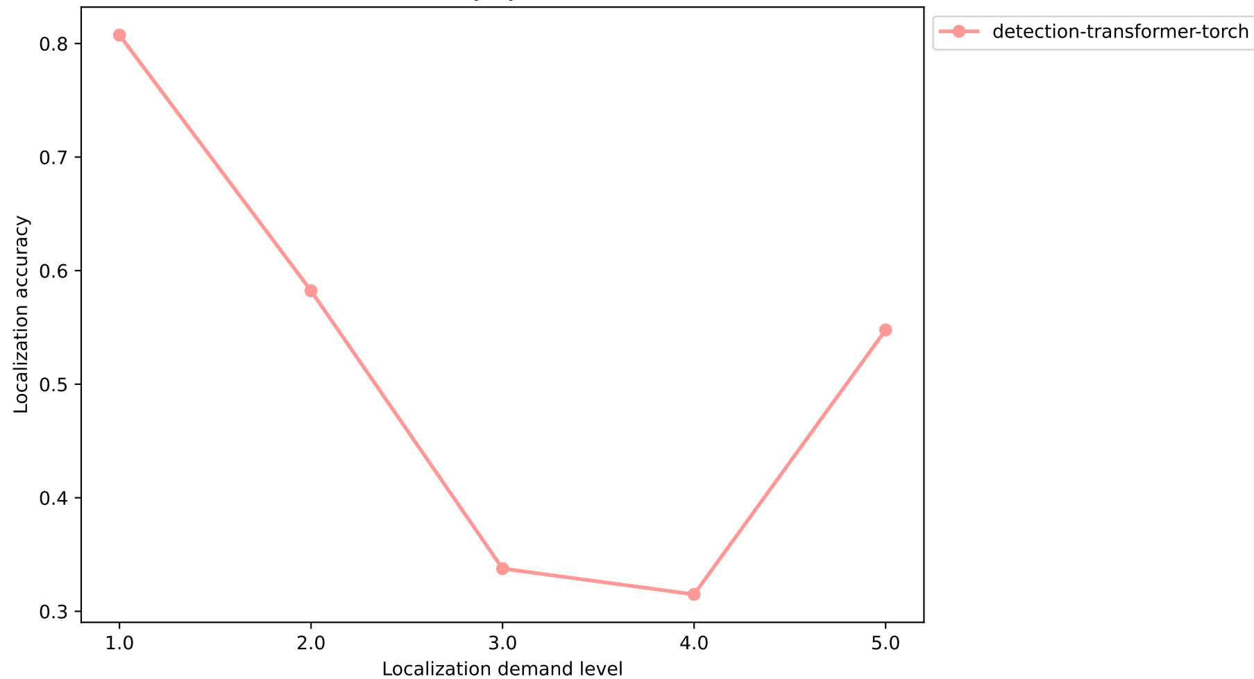
DETR Localization Accuracy by Localization Demand Level
