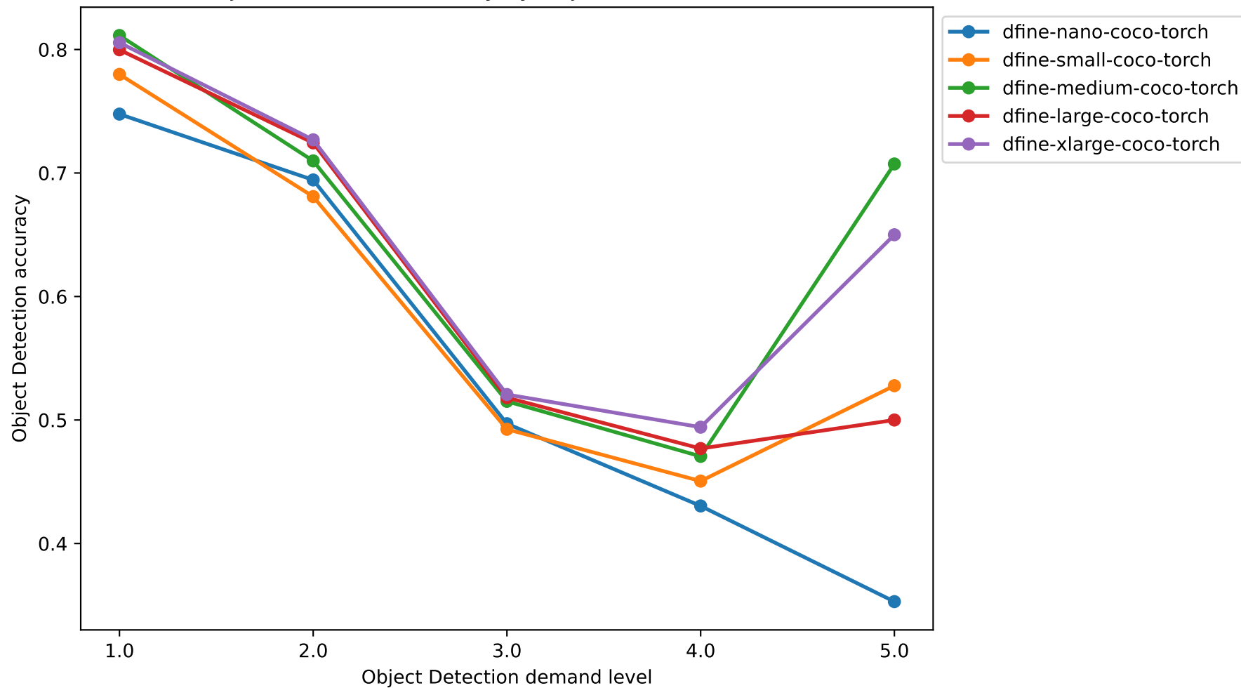
D-FINE Object Detection Accuracy by Object Detection Demand Level
