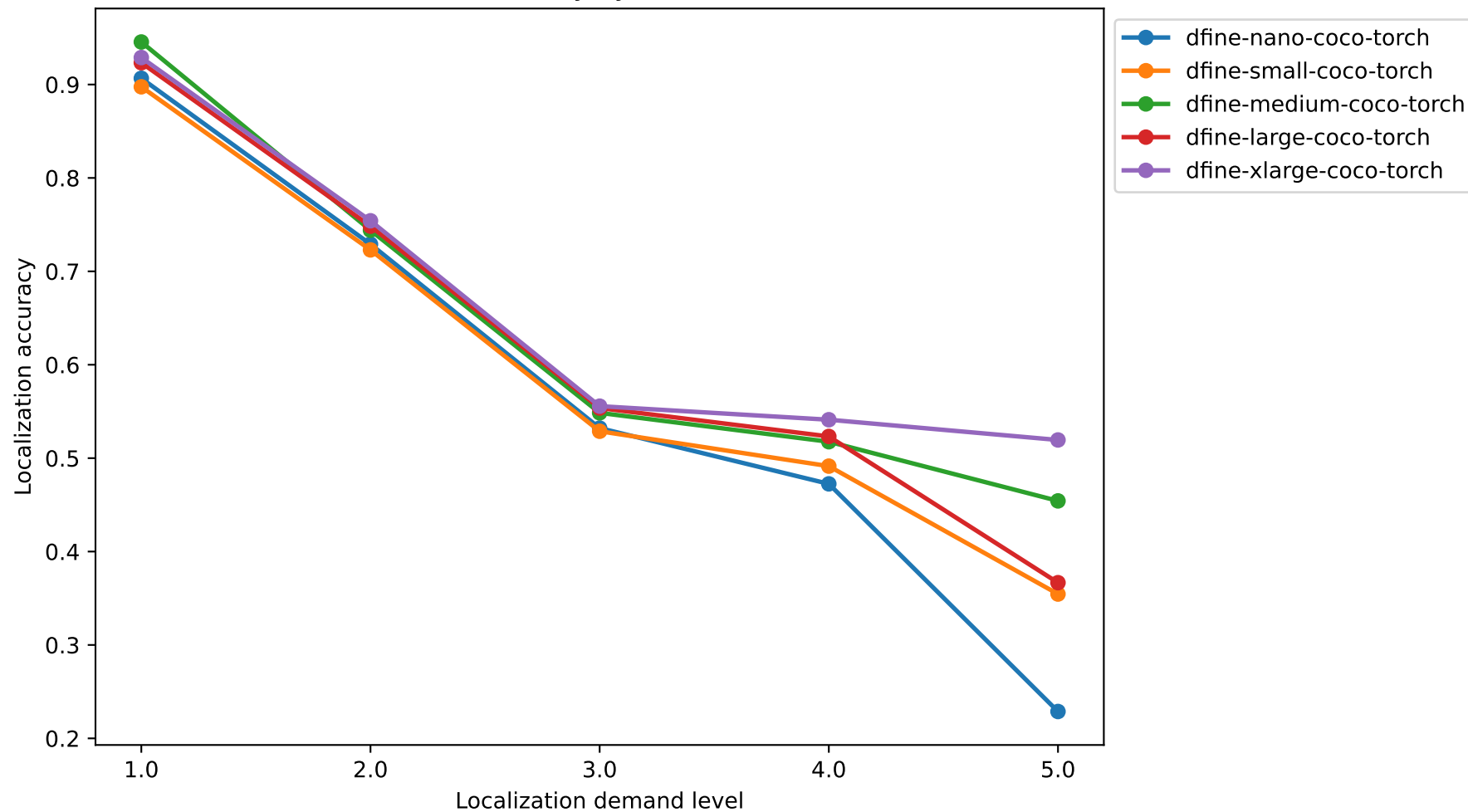
D-FINE Localization Accuracy by Localization Demand Level
