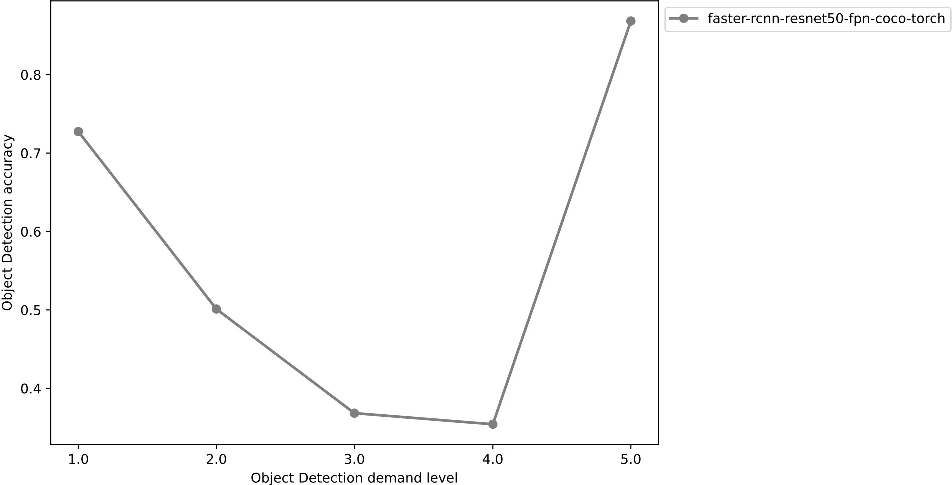
Faster R-CNN Object Detection Accuracy by Object Detection Demand Level
