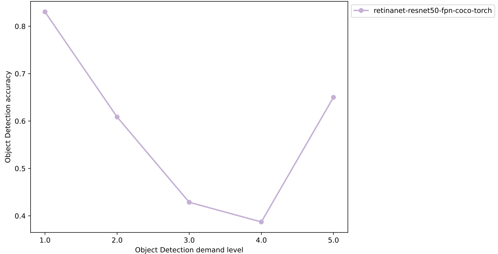
RetinaNet Object Detection Accuracy by Object Detection Demand Level
