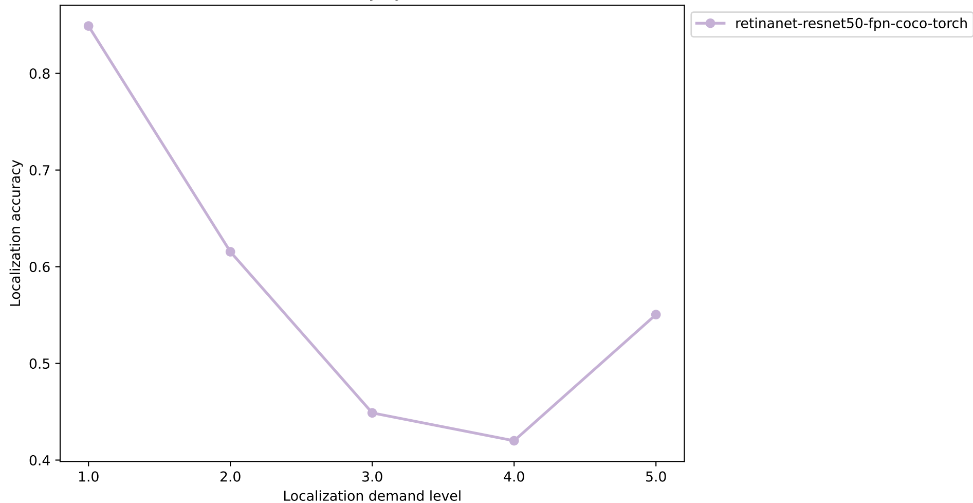
RetinaNet Localization Accuracy by Localization Demand Level
