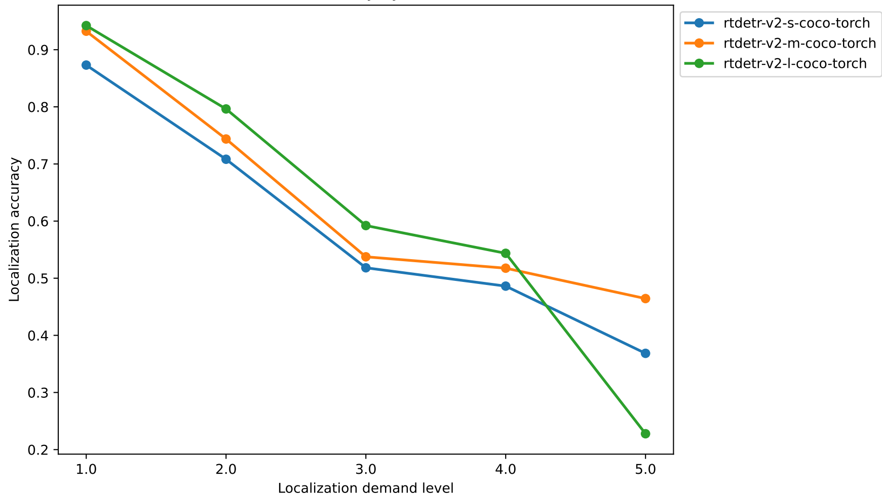
RT-DETRv2 Localization Accuracy by Localization Demand Level
