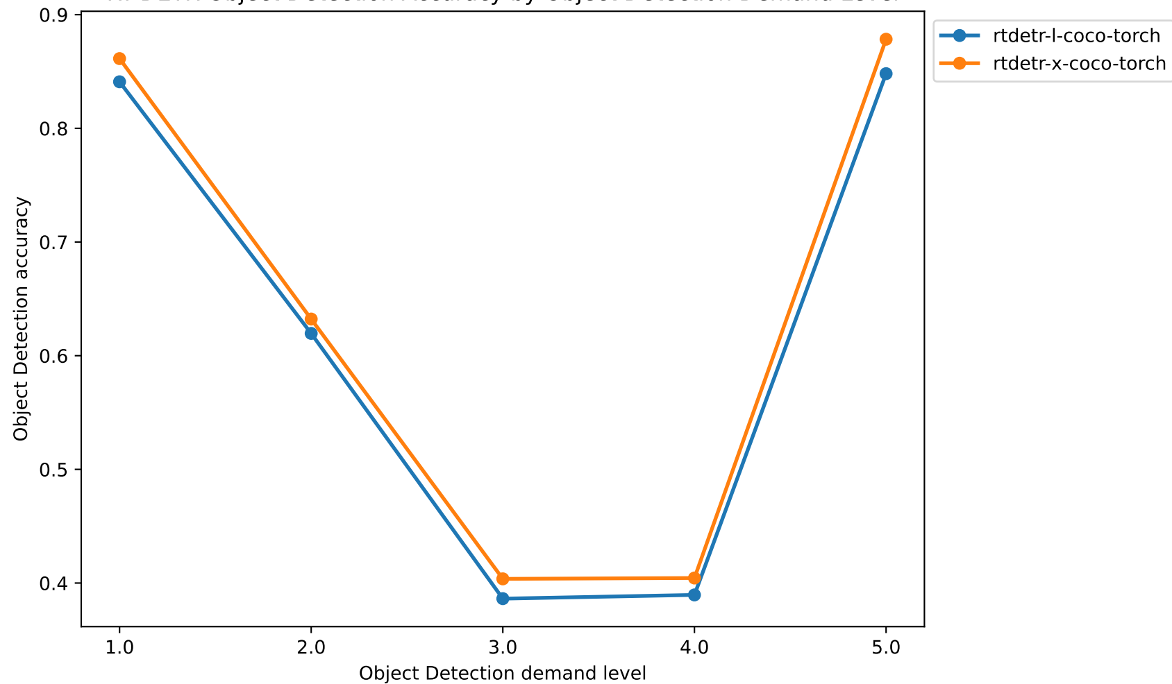
RT-DETR Object Detection Accuracy by Object Detection Demand Level
