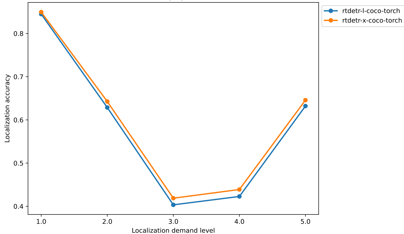
RT-DETR Localization Accuracy by Localization Demand Level
