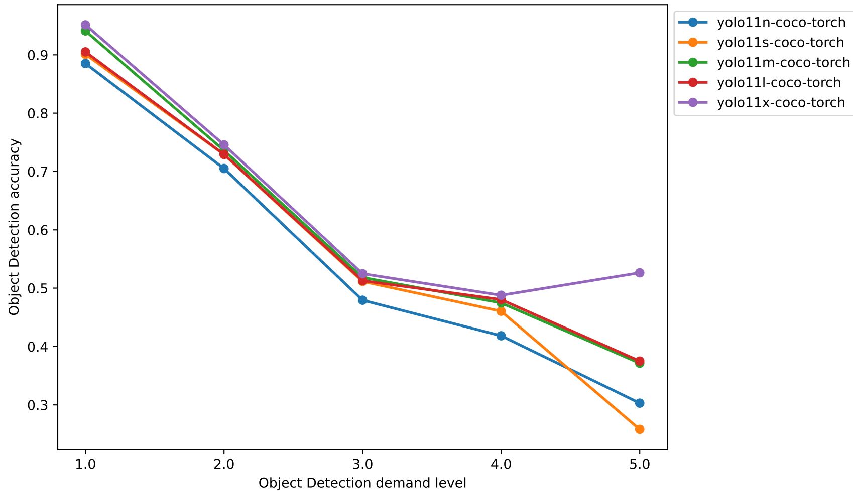
YOLO11 Object Detection Accuracy by Object Detection Demand Level
