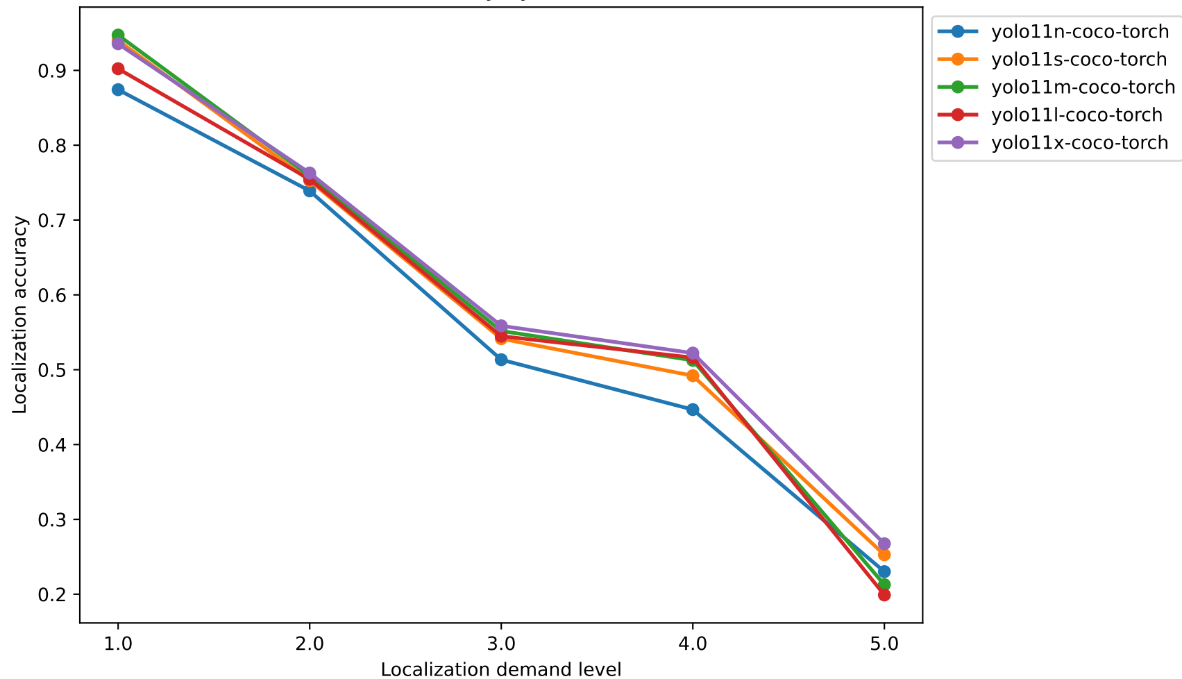
YOLO11 Localization Accuracy by Localization Demand Level
