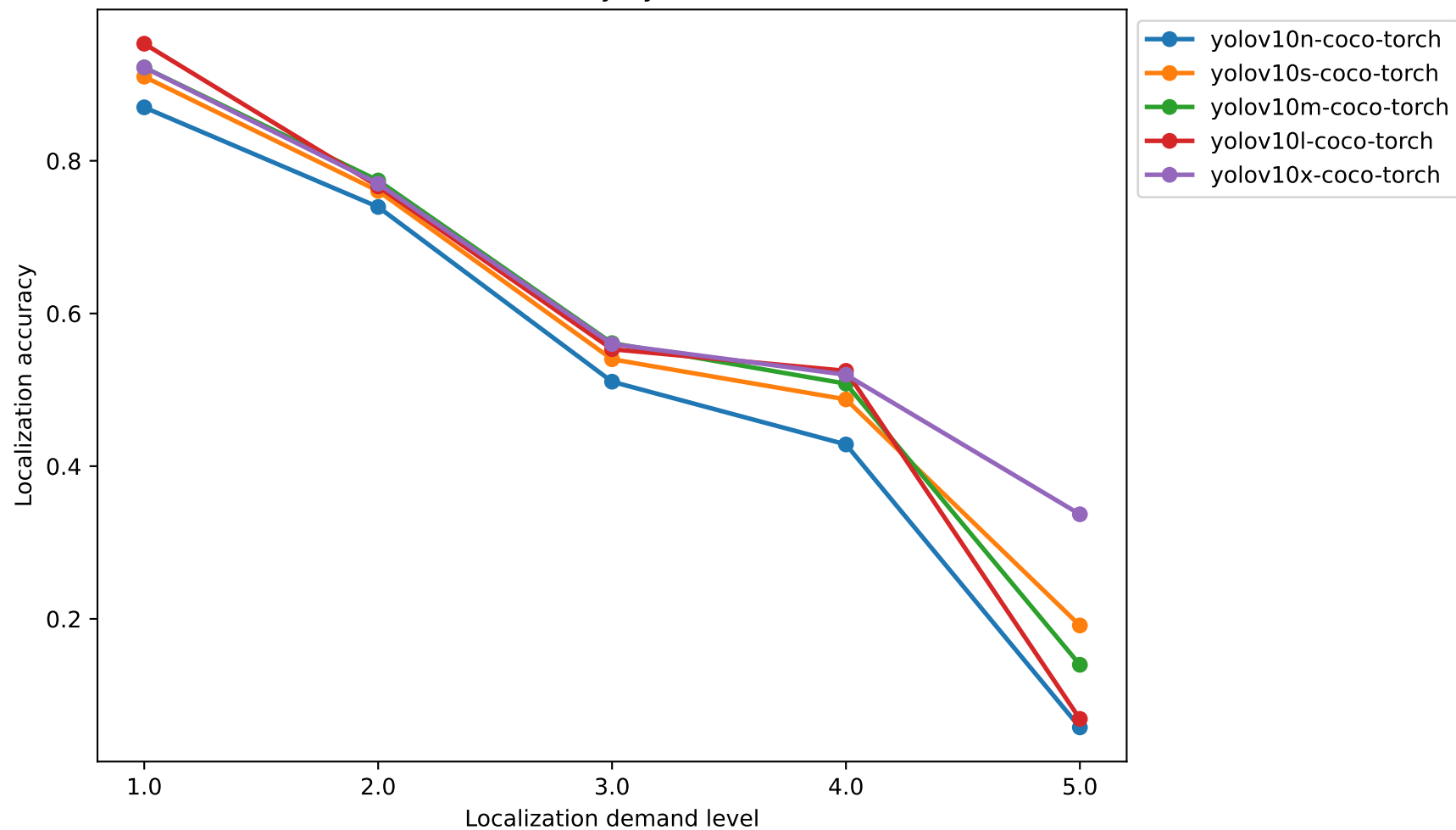
YOLOv10 Localization Accuracy by Localization Demand Level
