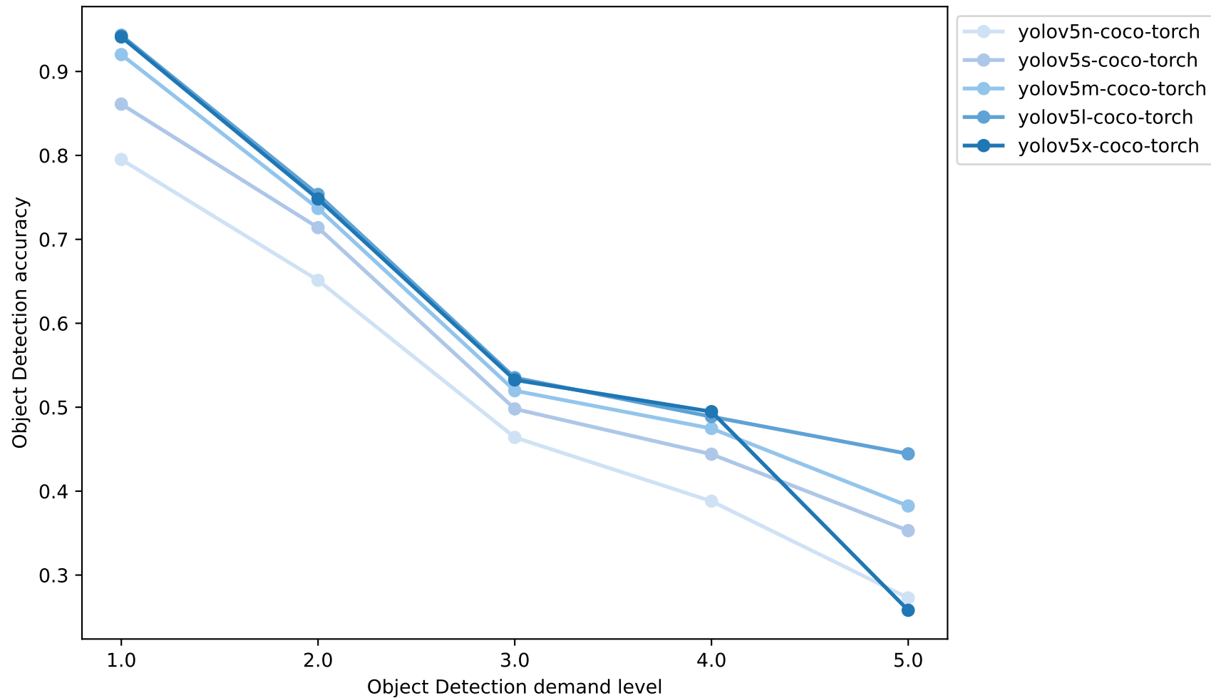
YOLOv5 Object Detection Accuracy by Object Detection Demand Level
