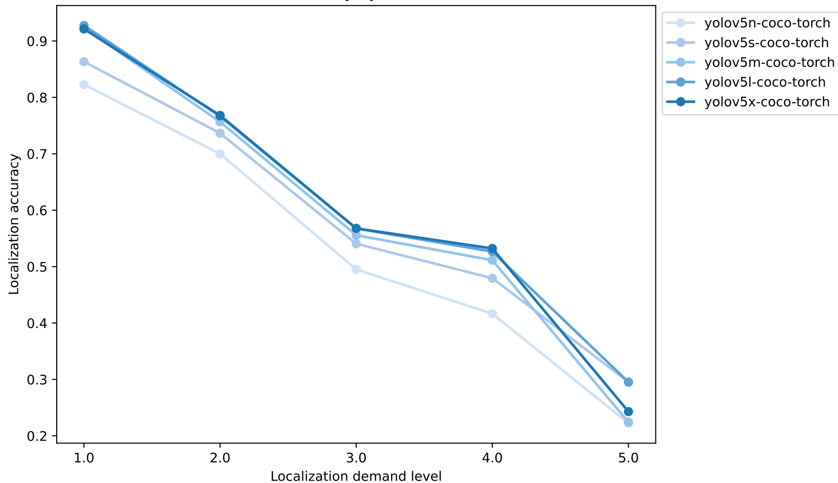
YOLOv5 Localization Accuracy by Localization Demand Level
