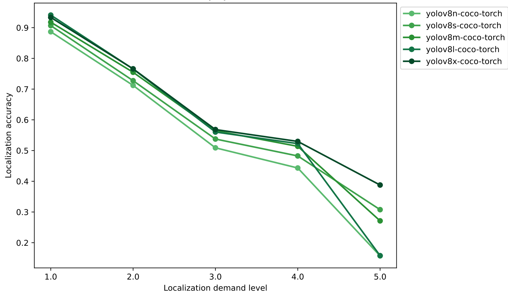
YOLOv8 Localization Accuracy by Localization Demand Level
