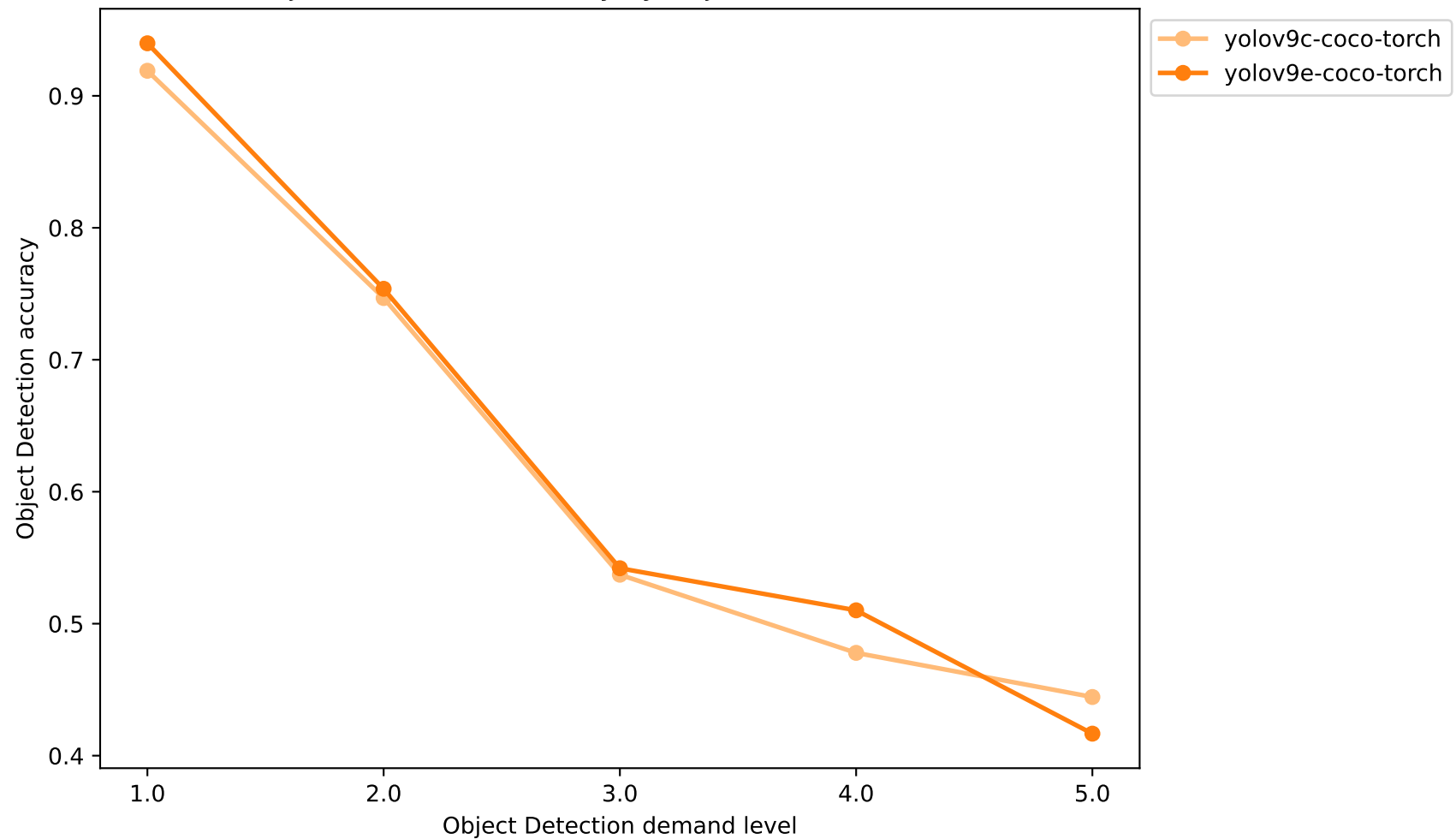
YOLOv9 Object Detection Accuracy by Object Detection Demand Level
