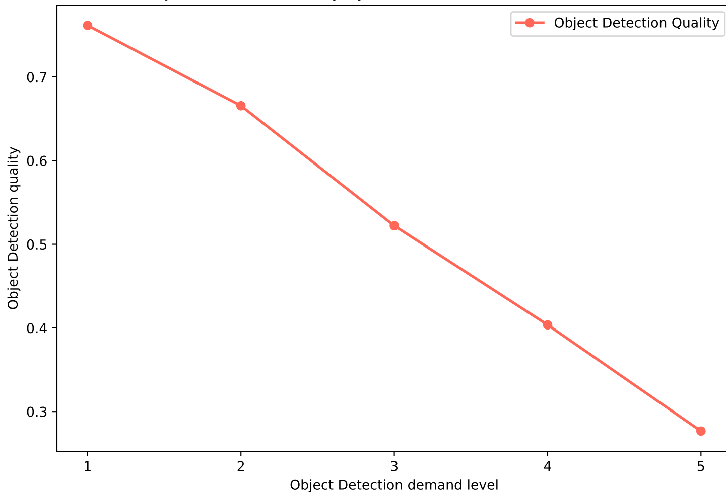
Mean Object Detection Quality by Demand Level — Zero-shot (calibration)
