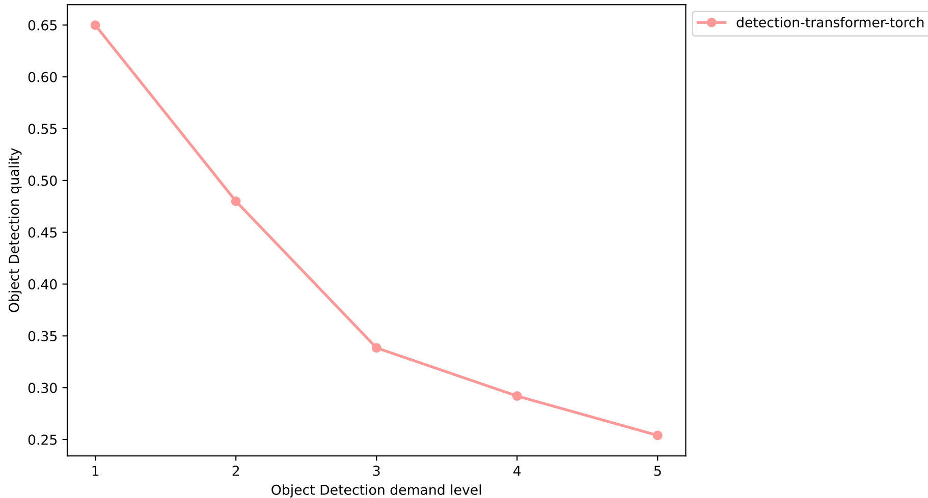
DETR Object Detection Quality by Demand Level — Zero-shot (calibration)
