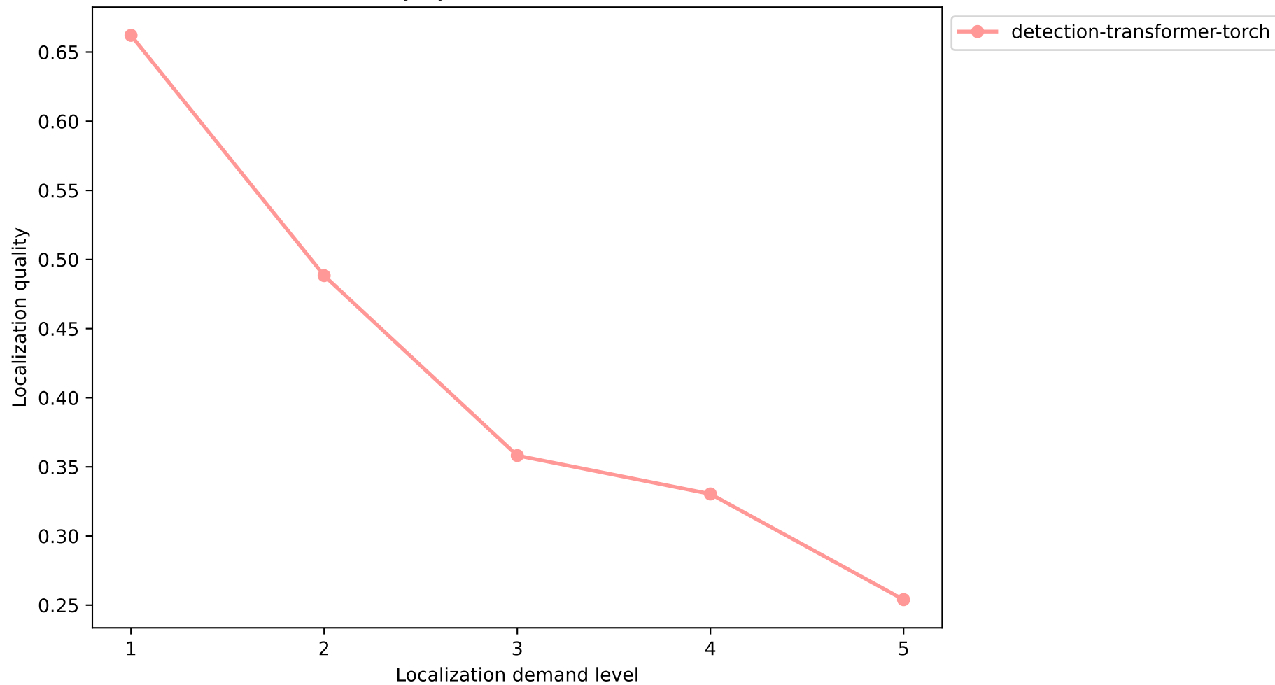
DETR Localization Quality by Demand Level — Zero-shot (calibration)
