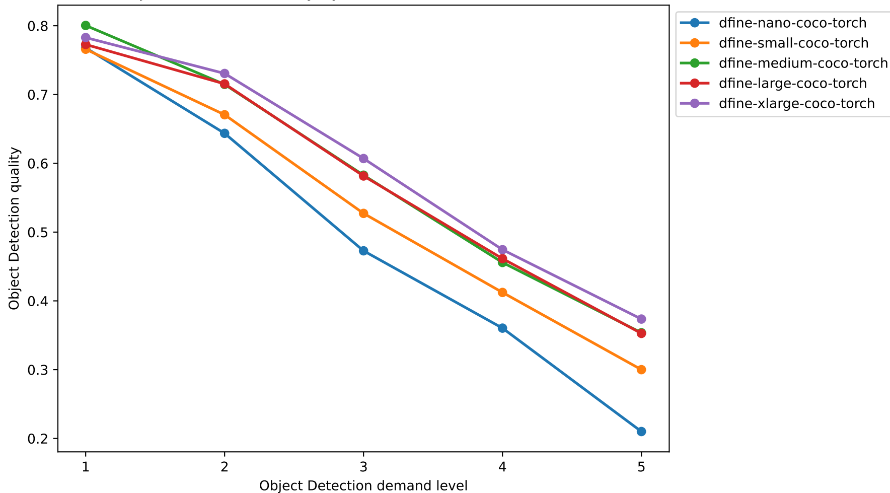
D-FINE Object Detection Quality by Demand Level — Zero-shot (calibration)
