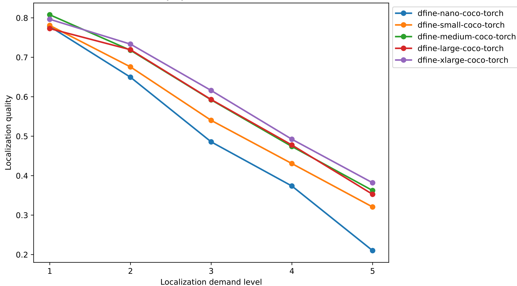
D-FINE Localization Quality by Demand Level — Zero-shot (calibration)
