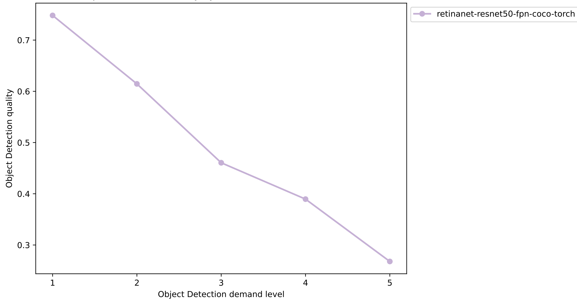
RetinaNet Object Detection Quality by Demand Level — Zero-shot (calibration)
