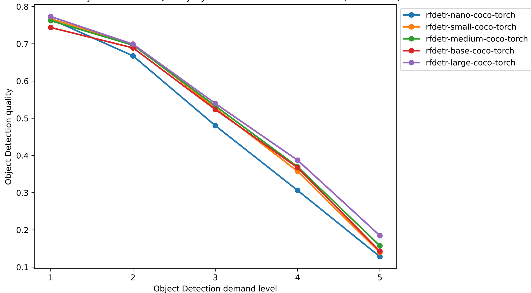
RF-DETR Object Detection Quality by Demand Level — Zero-shot (calibration)
