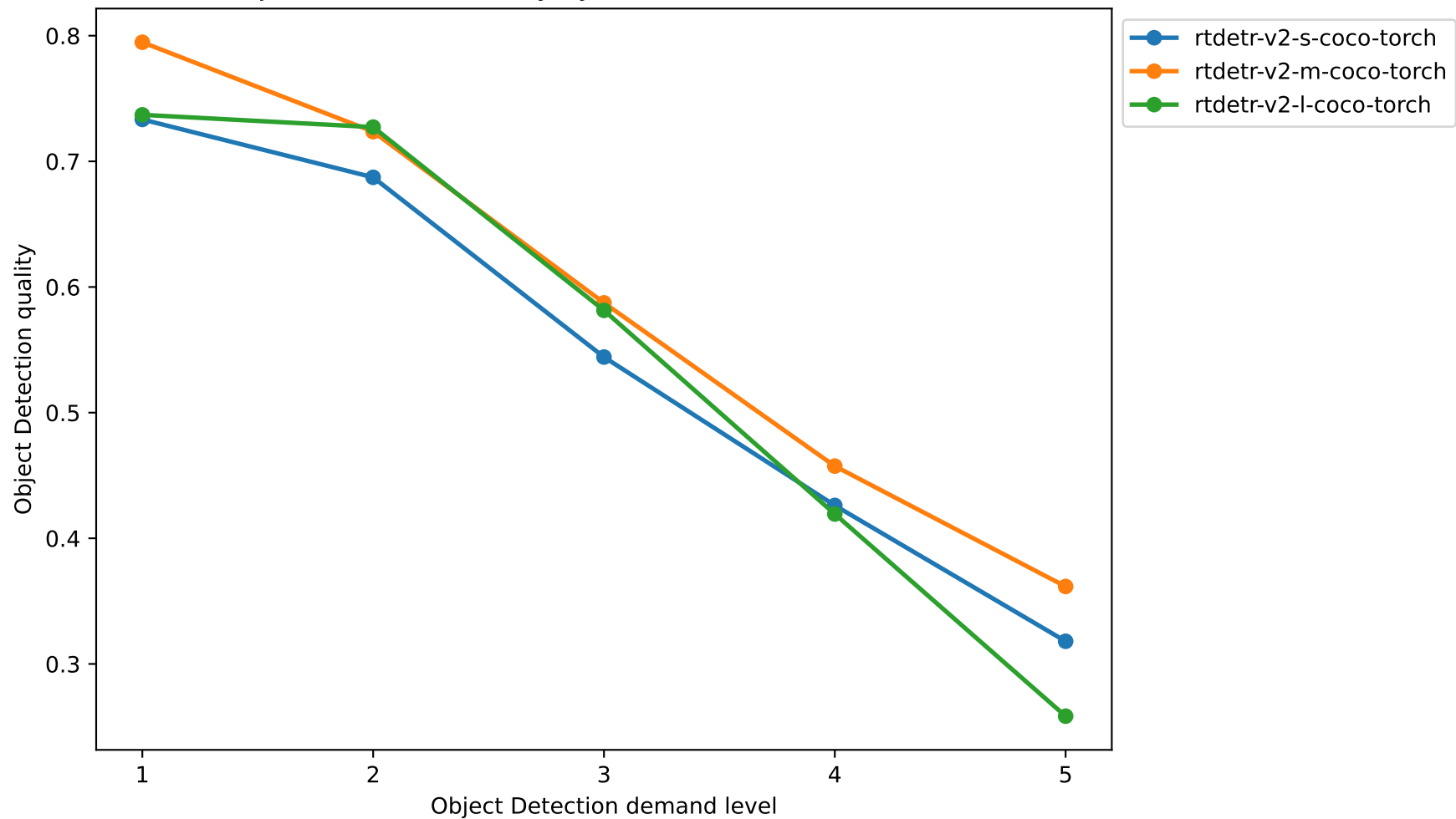
RT-DETRv2 Object Detection Quality by Demand Level — Zero-shot (calibration)
