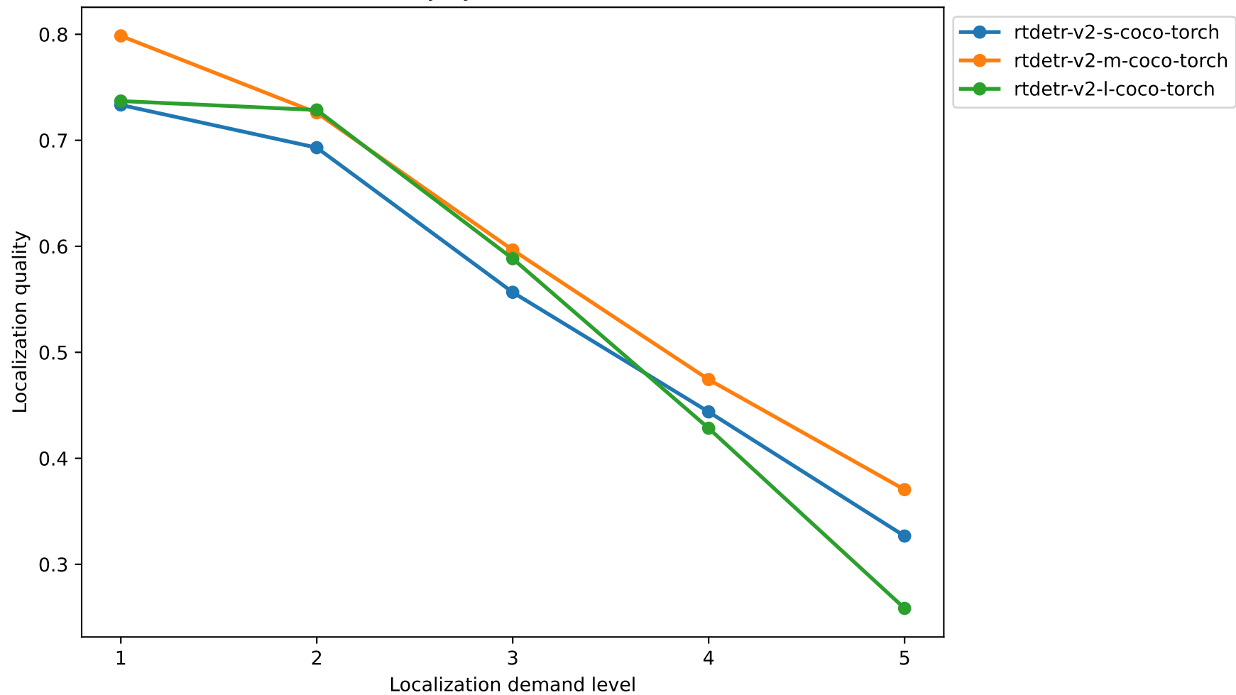
RT-DETRv2 Localization Quality by Demand Level — Zero-shot (calibration)
