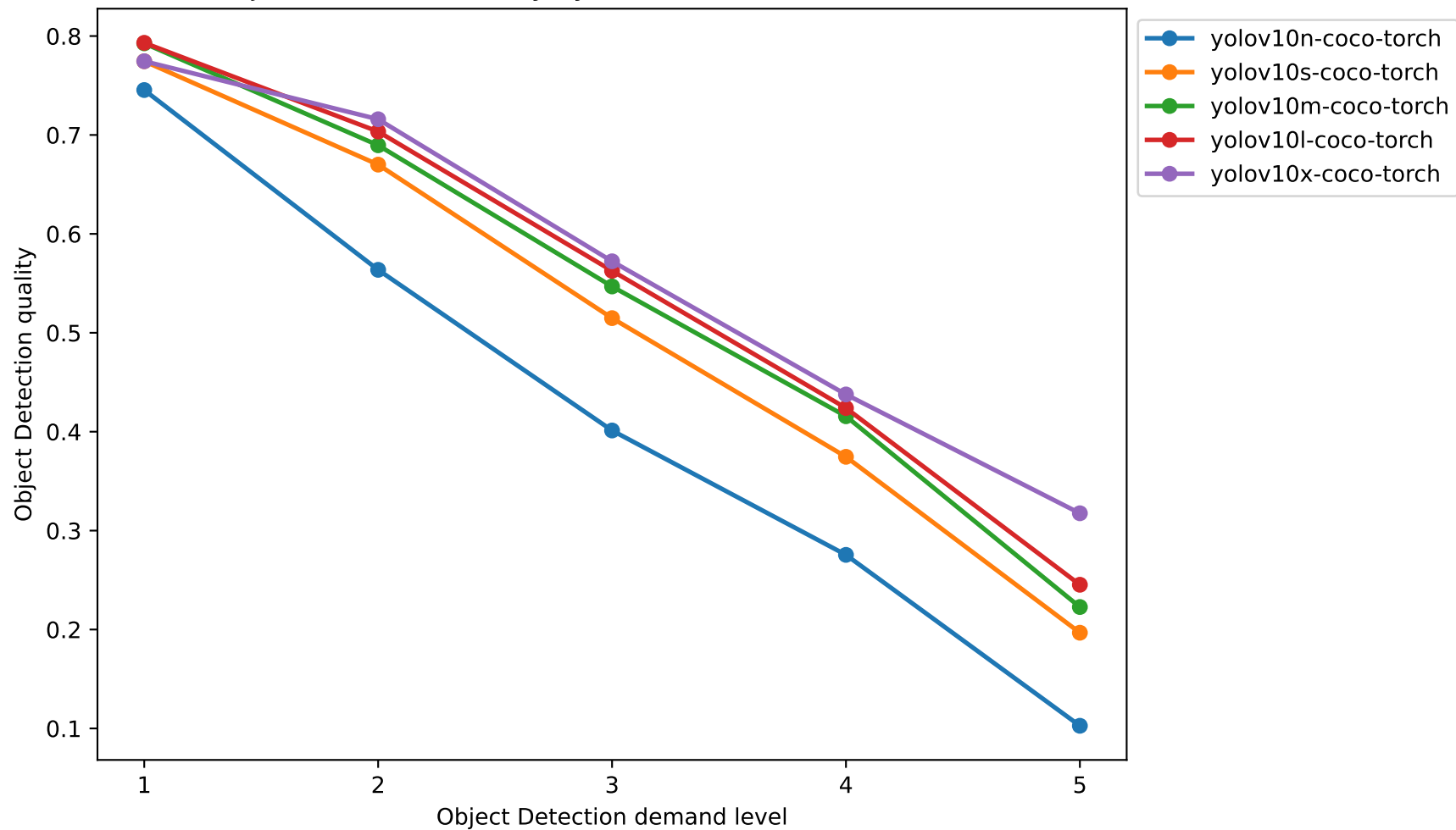
YOLOv10 Object Detection Quality by Demand Level — Zero-shot (calibration)
