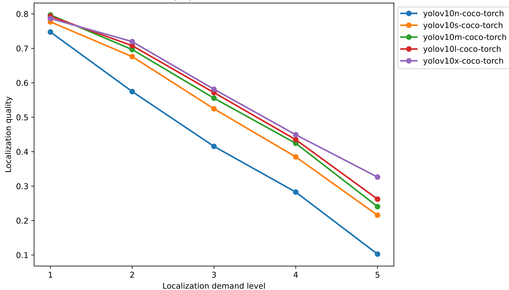
YOLOv10 Localization Quality by Demand Level — Zero-shot (calibration)
