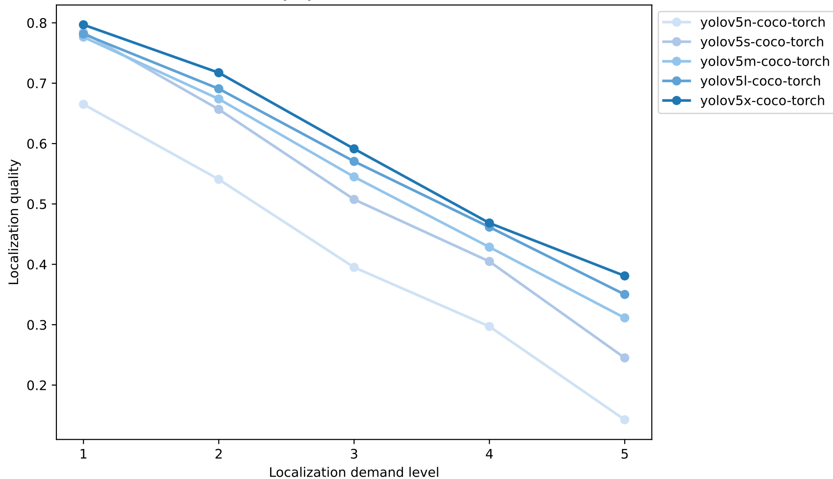
YOLOv5 Localization Quality by Demand Level — Zero-shot (calibration)
