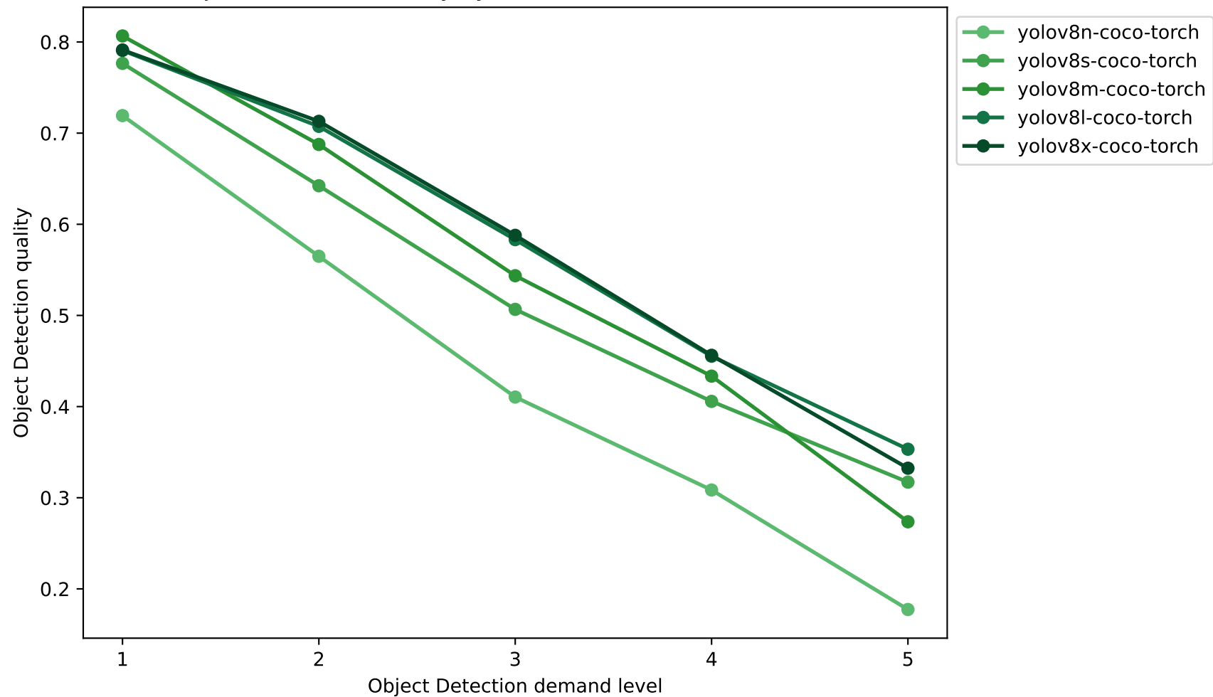
YOLOv8 Object Detection Quality by Demand Level — Zero-shot (calibration)
