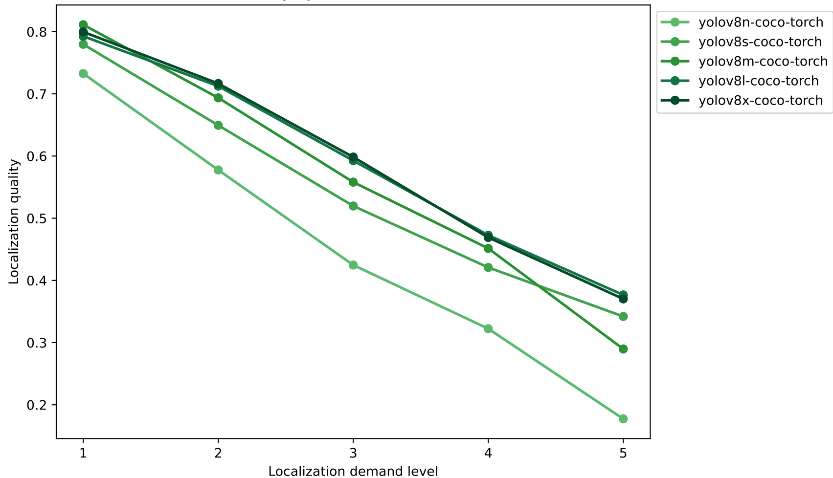
YOLOv8 Localization Quality by Demand Level — Zero-shot (calibration)
