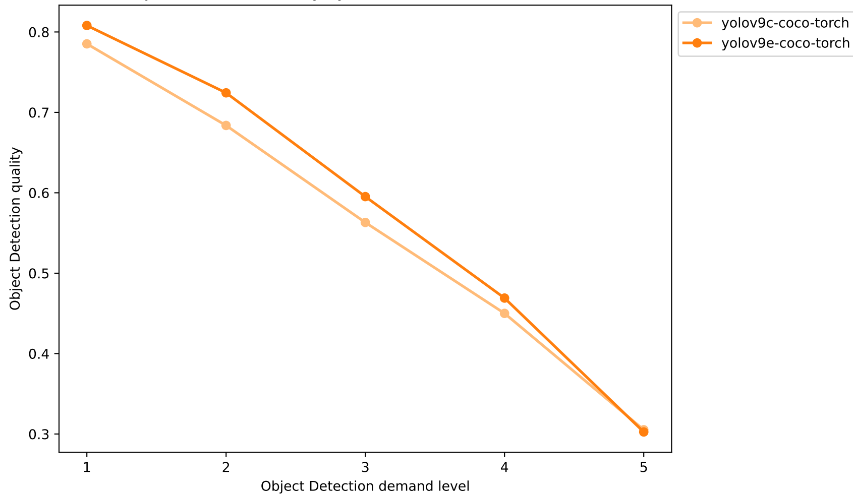
YOLOv9 Object Detection Quality by Demand Level — Zero-shot (calibration)
