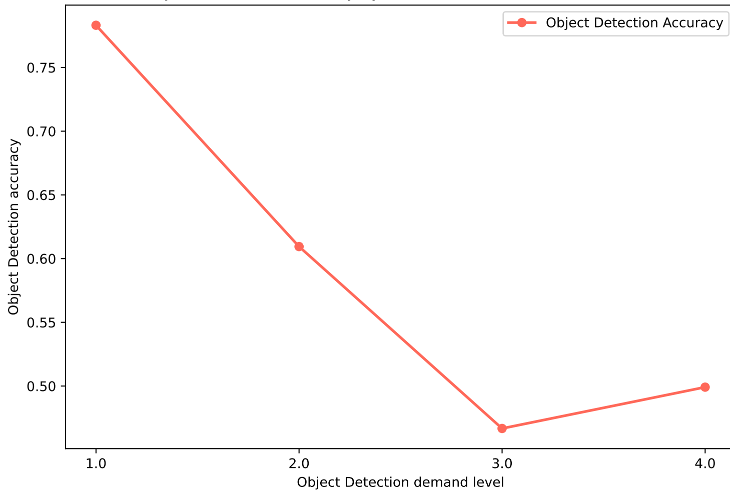
Mean Object Detection Accuracy by Demand Level — Zero-shot (calibration)
