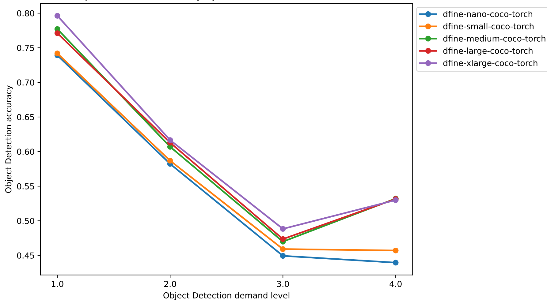
D-FINE Object Detection Accuracy by Demand Level — Zero-shot (calibration)
