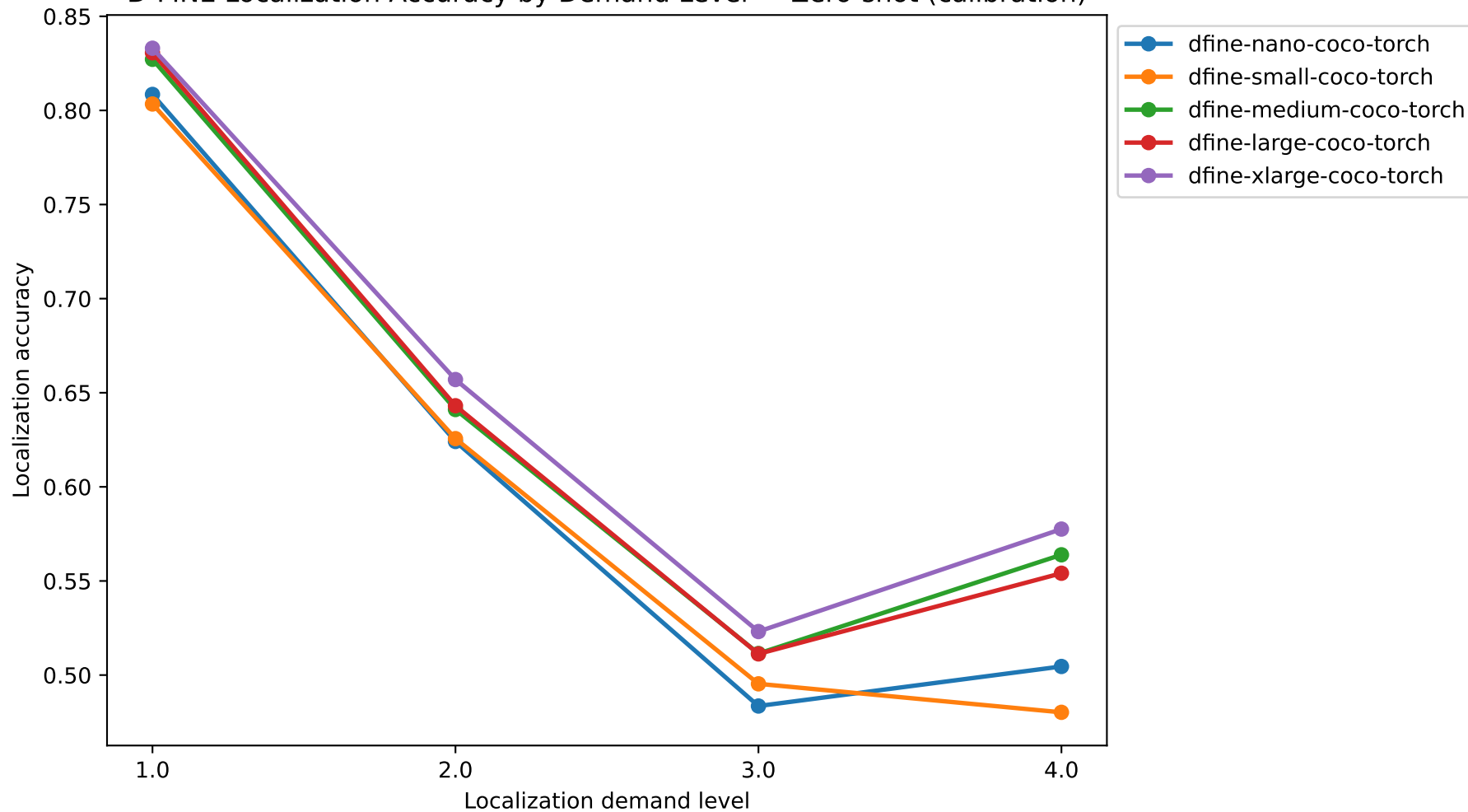
D-FINE Localization Accuracy by Demand Level — Zero-shot (calibration)
