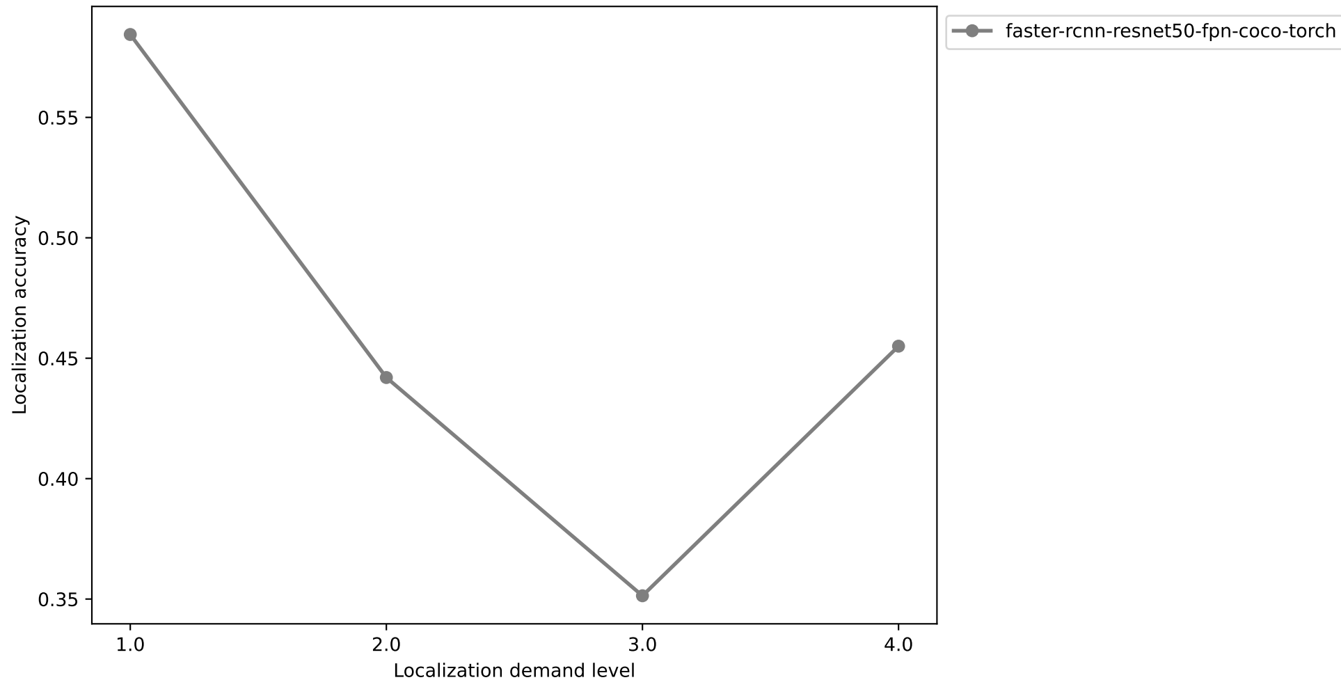
Faster R-CNN Localization Accuracy by Demand Level — Zero-shot (calibration)
