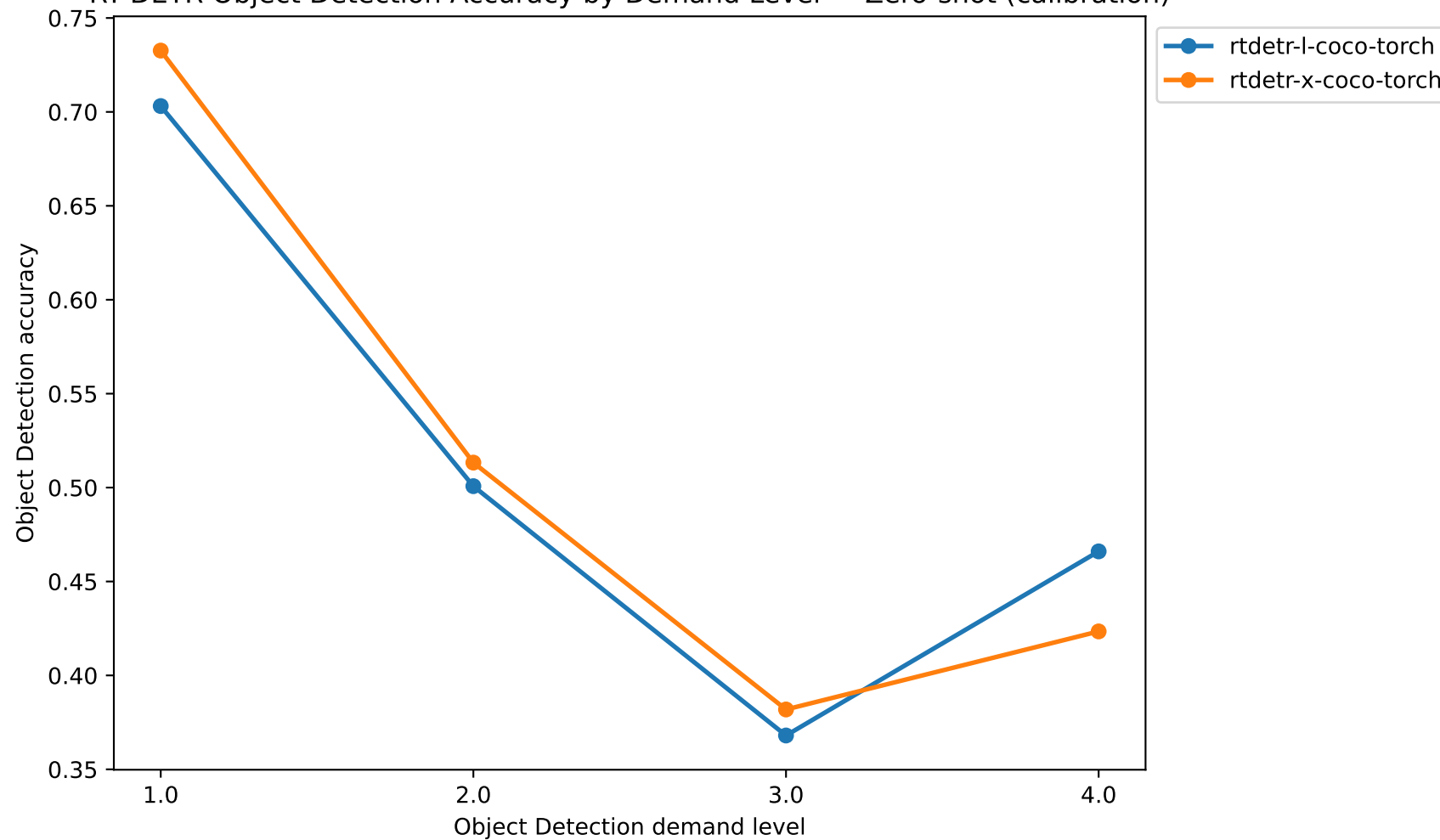
RT-DETR Object Detection Accuracy by Demand Level — Zero-shot (calibration)
