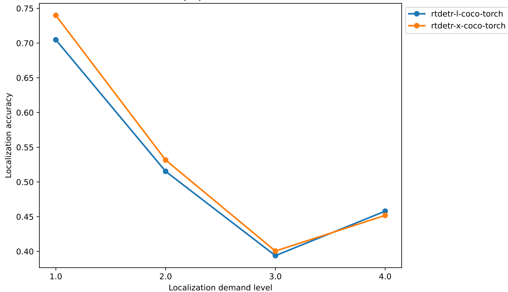
RT-DETR Localization Accuracy by Demand Level — Zero-shot (calibration)
