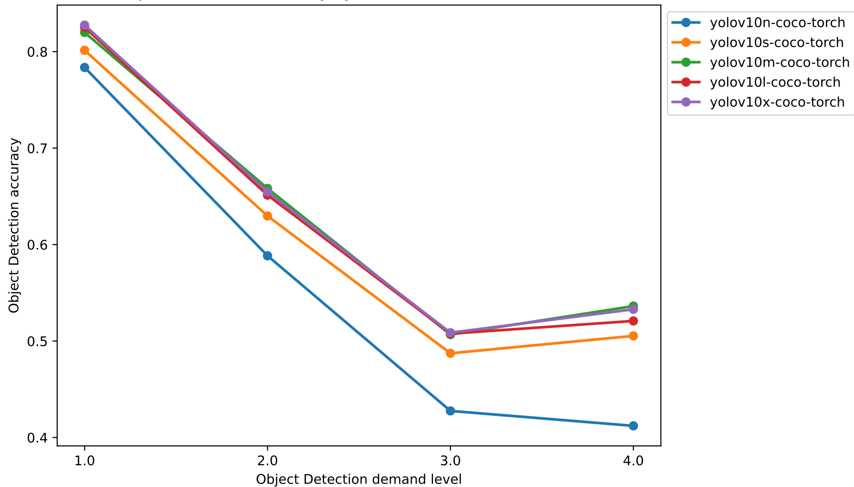
YOLOv10 Object Detection Accuracy by Demand Level — Zero-shot (calibration)
