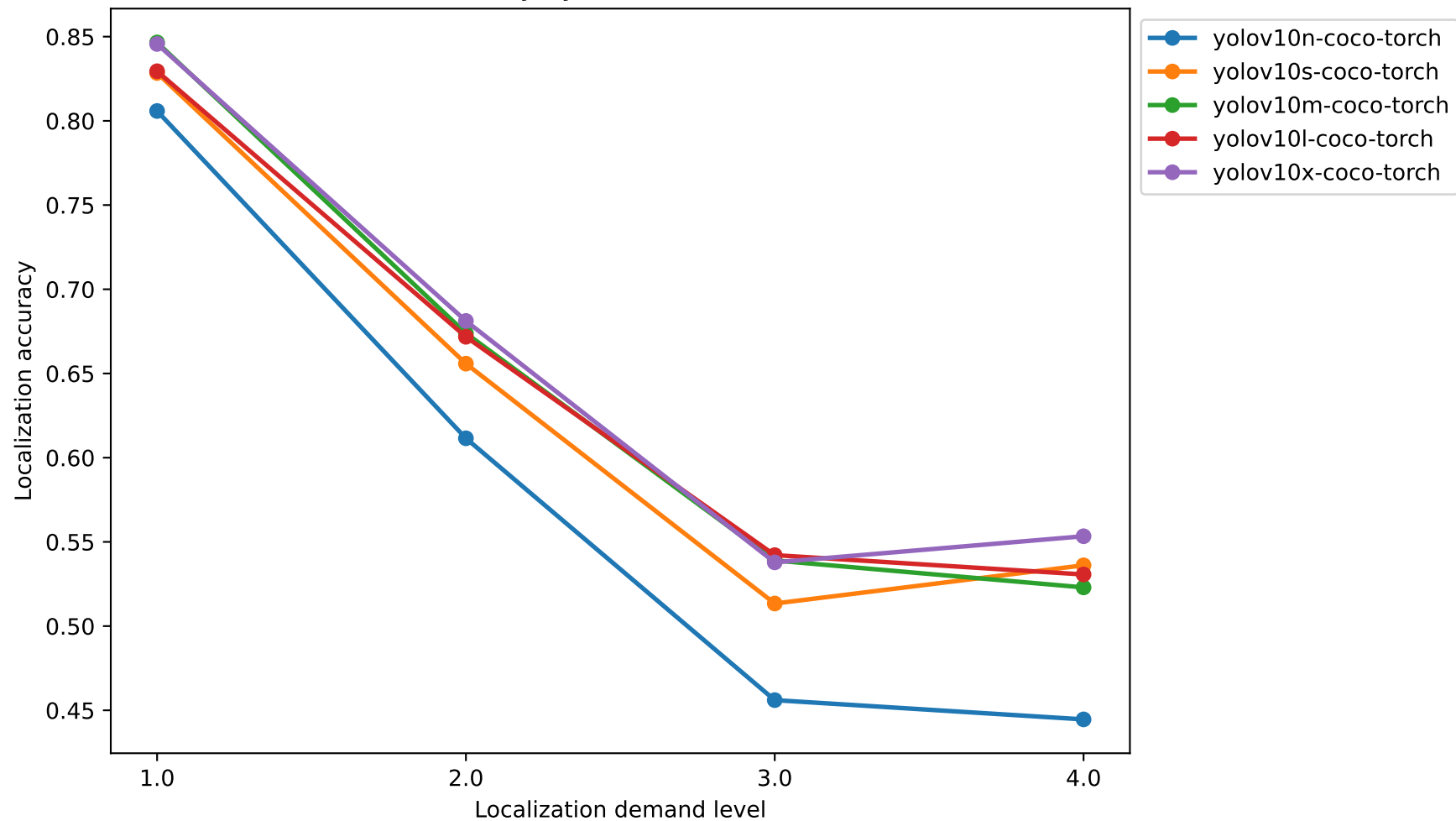
YOLOv10 Localization Accuracy by Demand Level — Zero-shot (calibration)
